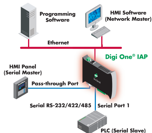
Diagram 2: Digi Pass-Through Port Solution
